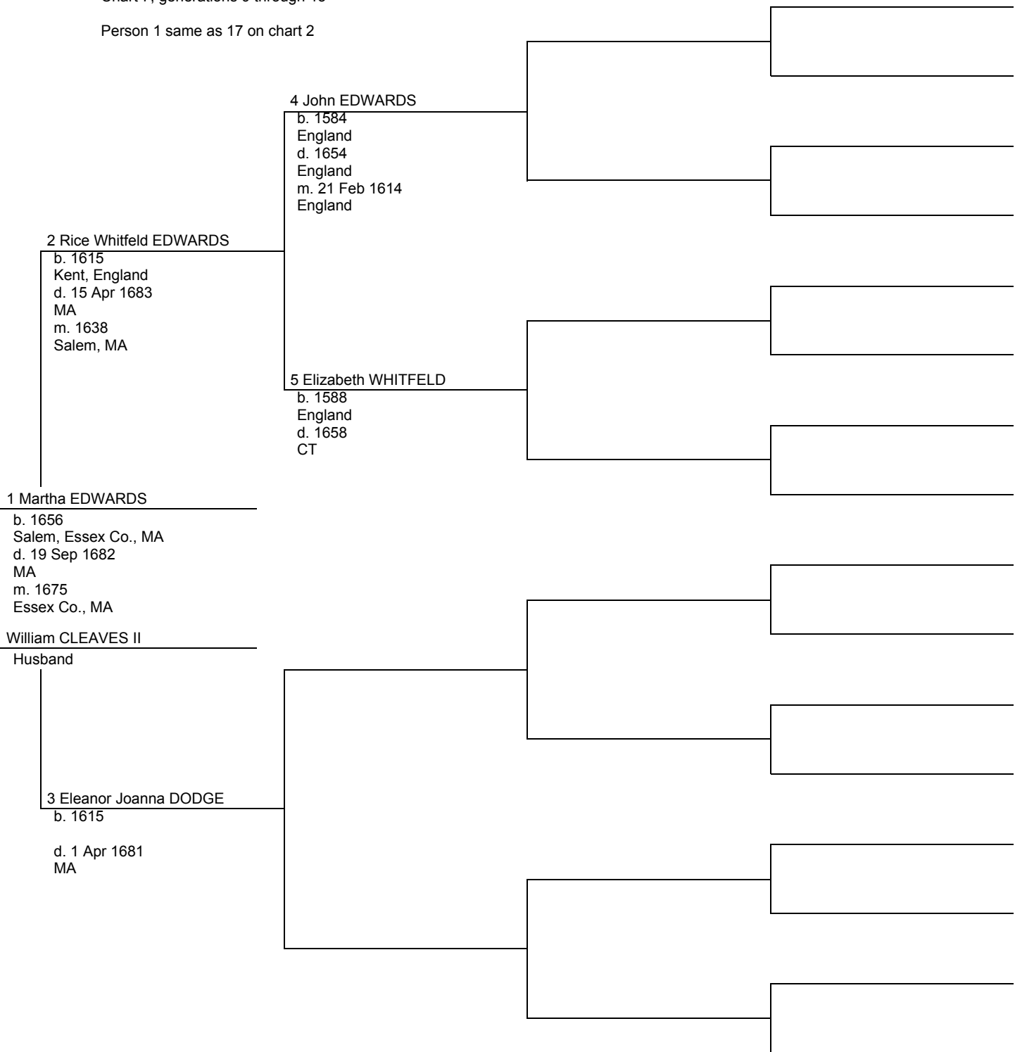
Chart 7, generations 9 through 13
